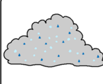
condensation
