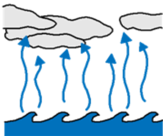
evaporation
